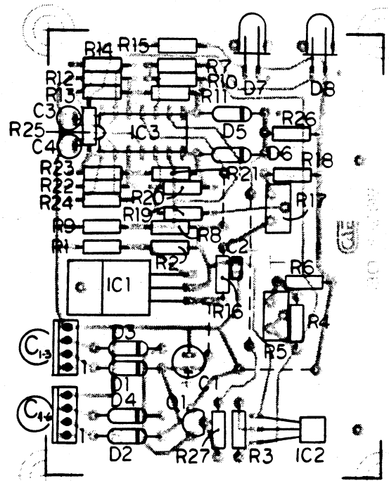
FOIL SIDE VIEW OT/OV PCA layout
